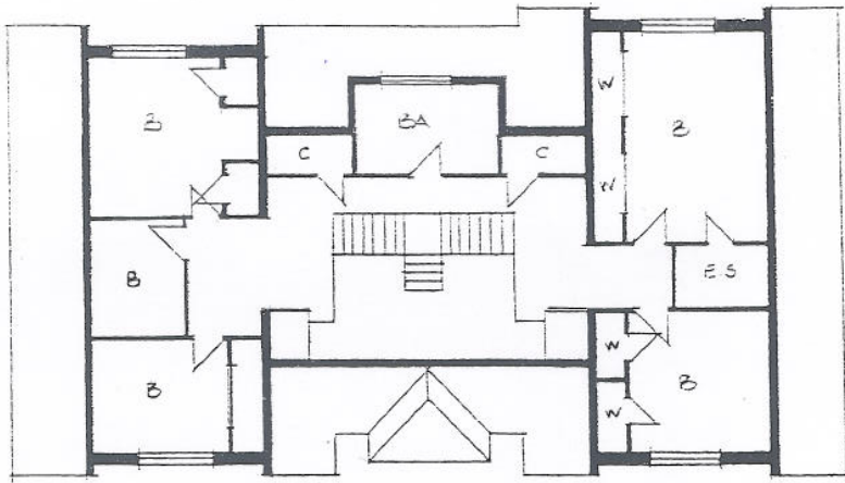
First Floor Plan 1:200
